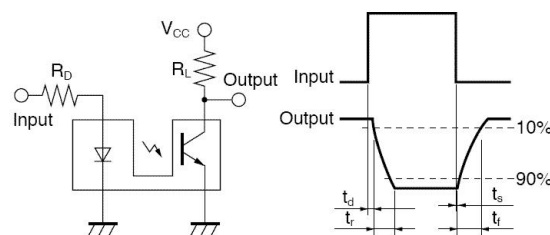
Fig.4 Test Circuit for Response Time
