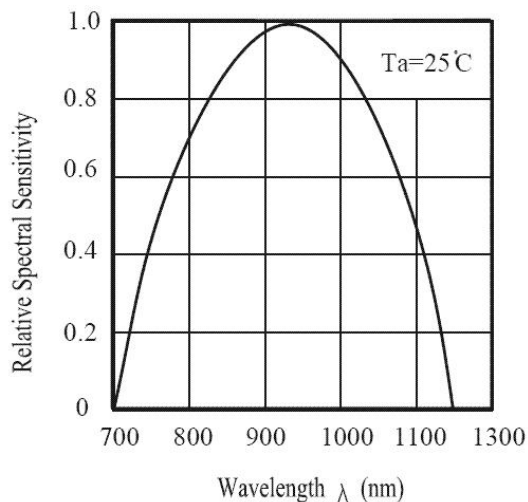
Fig.5 Spectral Sensitivity for PT
