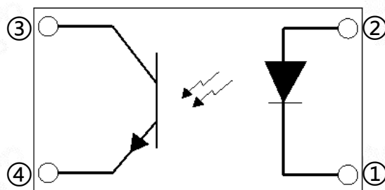
Pin Configuration
