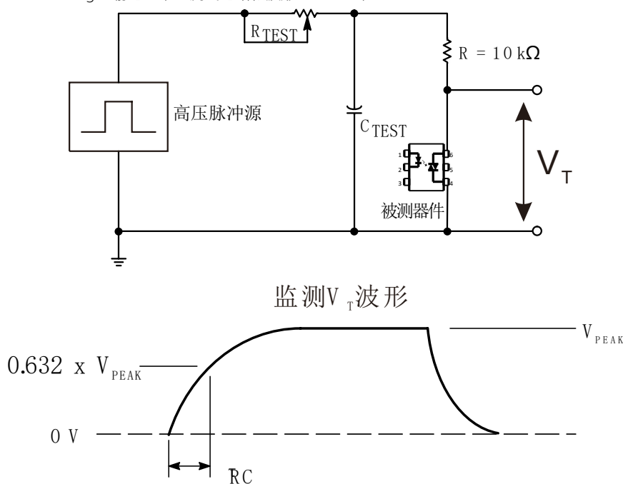
Fig.11 静态 dv/dt 测试电路和波形 Static dv/dt test circuit and waveform
