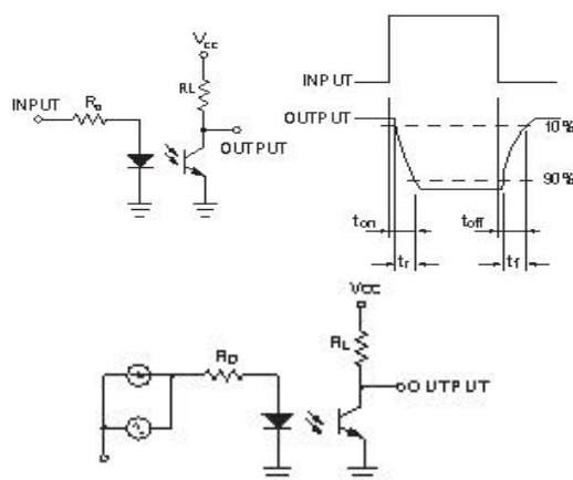
Fig.10 Test Circuits
