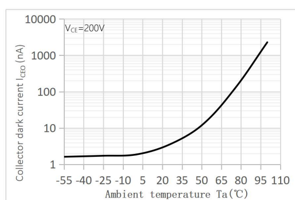
Fig.6 Collector Dark Current vs Ambient Temperature
