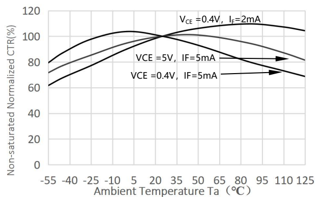
Fig.6 Relative Current Transfer Ratio vs. Ambient Temperature
