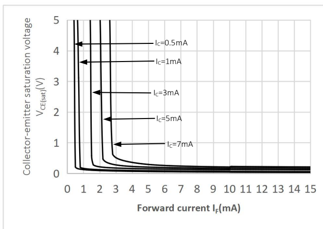
Fig.11 Collector-emitter Saturation Voltage vs Forward Current
