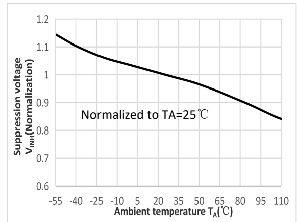
Fig.10 Suppression voltage vs Ambient temperature
