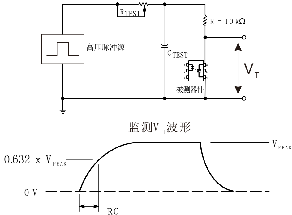
Fig.11 静态 dv/dt 测试电路和波形 Static dv/dt test circuit and waveform
