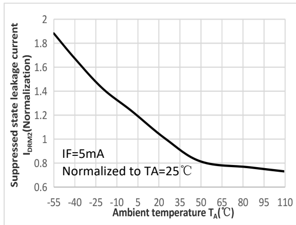
Fig.9 Suppressed state leakage current vs Ambient temperature
