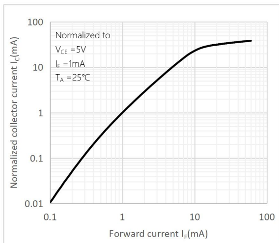
Fig.5 Normalized collector current vs Forward current
