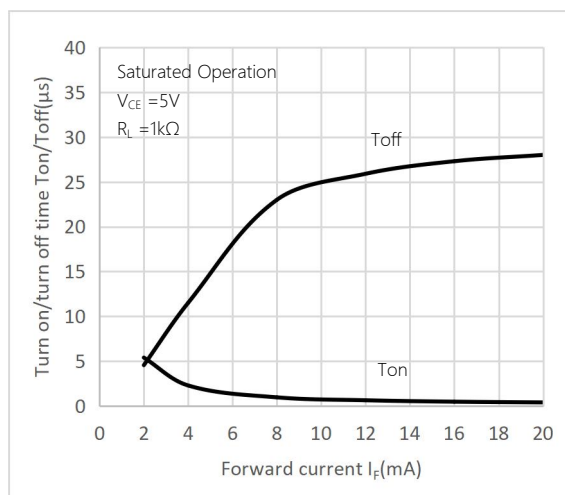
Fig.10 Turn on/Turn off time vs Forward current
