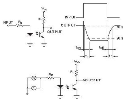
Fig.10 Test Circuits
