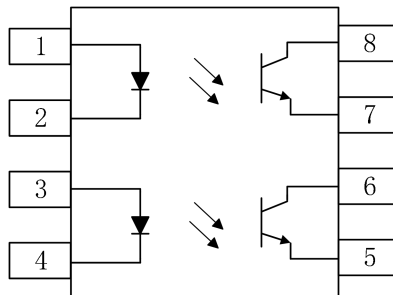
Pin Configuration
