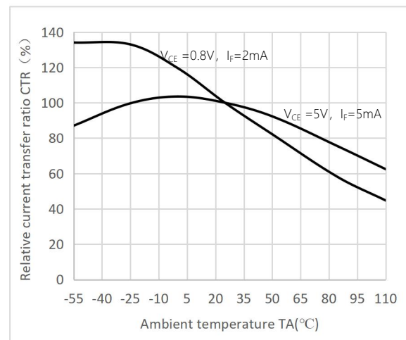
Fig.6 Relative Current Transfer Ratio vs. Ambient Temperature
