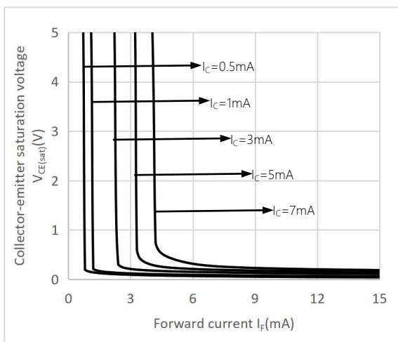
Fig.11 Collector-emitter Saturation Voltage vs Forward Current
