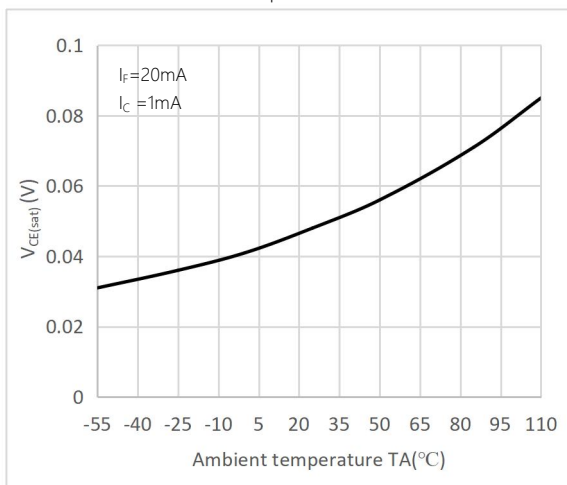
Fig.7 Collector-emitter Saturation Voltage vs. Ambient Temperature
