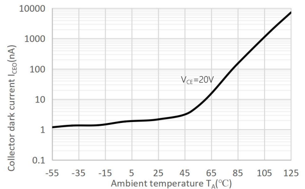
Fig.6 Collector Dark Current vs Ambient Temperature
