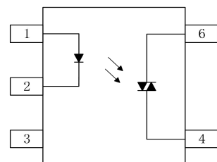
Pin Configuration
