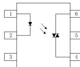
Pin Configuration
