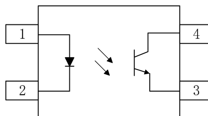
Pin Configuration
