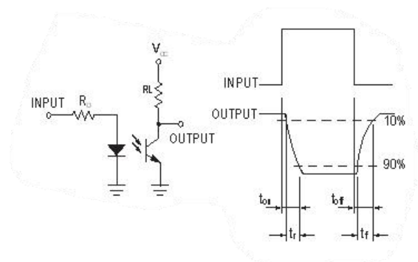
Fig.11 Switching Time Test Circuit & Wave forms
