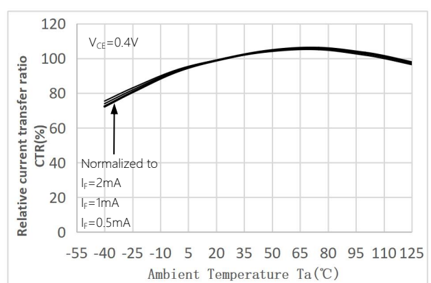
Fig.6 Relative Current Transfer Ratio vs.Ambient Temperature
