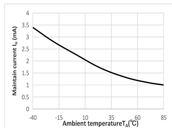
Fig.6 Maintain current vs Ambient temperature
