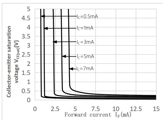
Fig.11 Collector-emitter Saturation Voltage vs Forward Current
