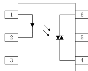
Pin Configuration
