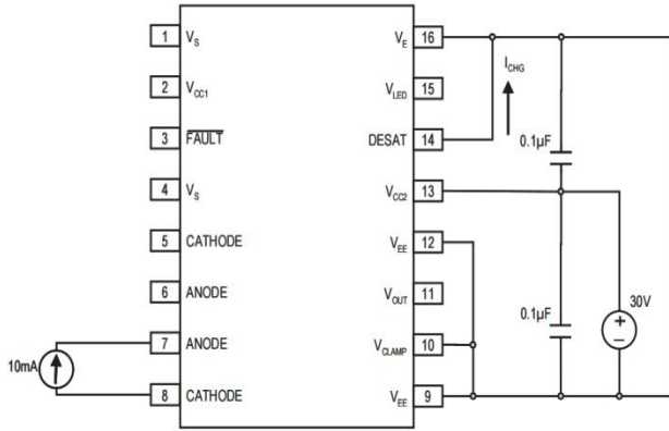
Fig 29. T_{PLH} , T_{PHL} , T_{fr} , T_{rr} Test Circuit
