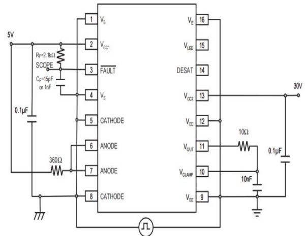
Fig 32. CMR Test Circuit LED2 on
