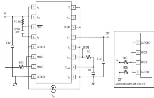
Fig 34. CMR Test circuit LED1 off
