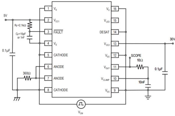
Fig 33. CMR Test Circuit LED1 on
