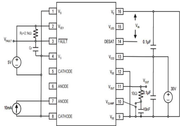
Fig 32. CMR Test Circuit LED2 on
