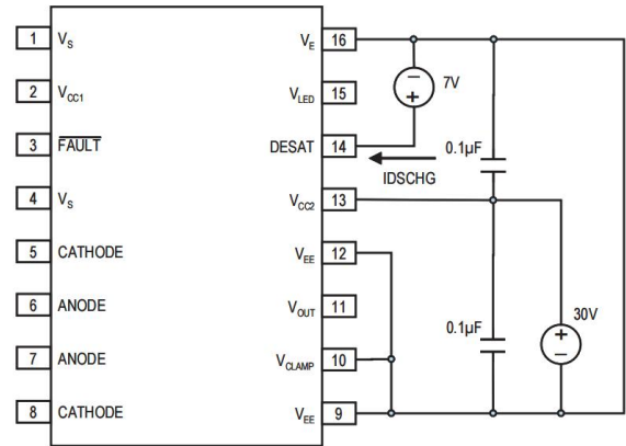
Fig 30. T_{DESAT} Fault Test Circuit
