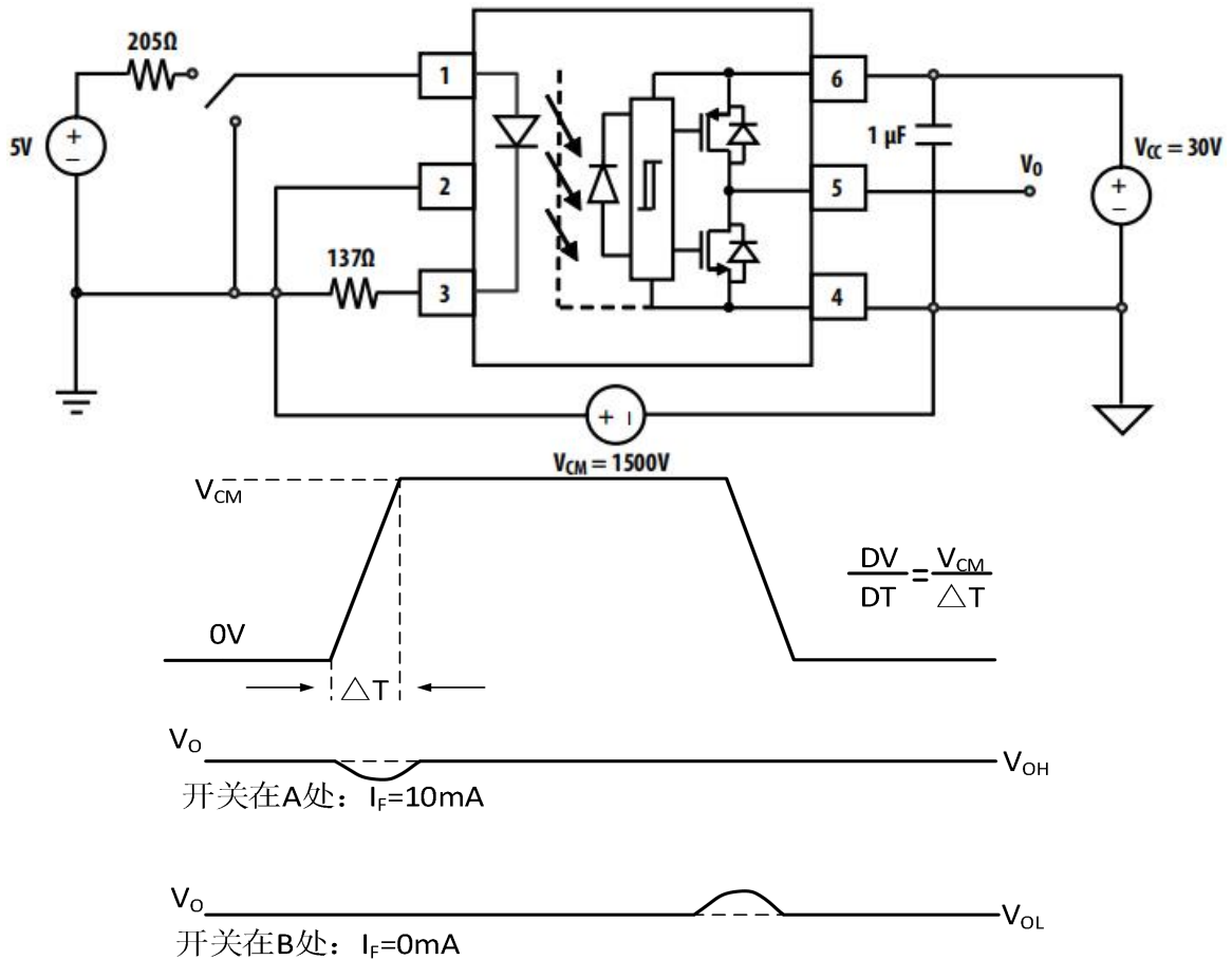
Figure.19 CMR Test Circuit
