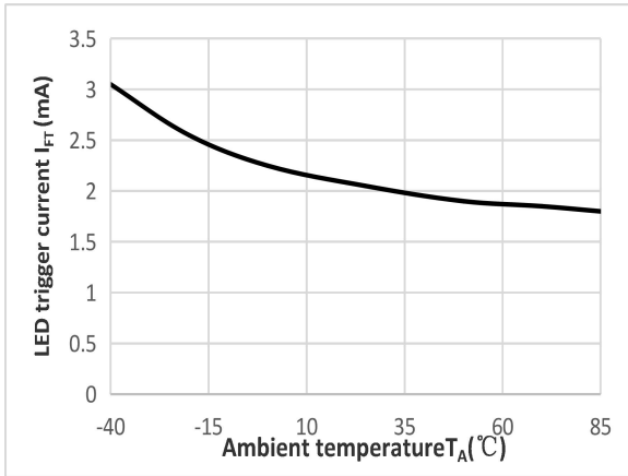
Fig.3 LED trigger current vs Ambient temperature
