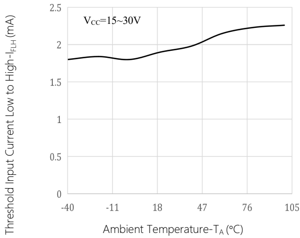
Fig.7 Threshold Input Current Low to High vs Ambient Temperature
