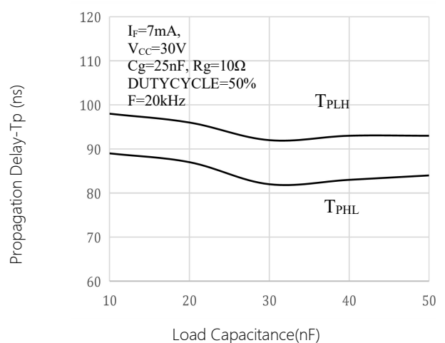
Fig.12 Propagation Delay vs. Load Capacitance
