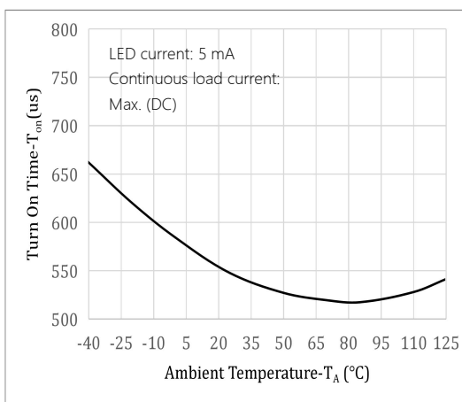
Fig.5 Turn On Time vs. Ambient Temperature Characteristics
