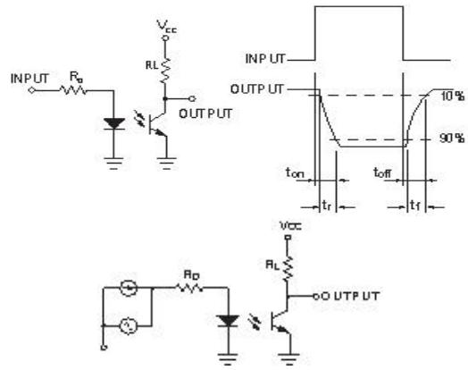
Fig.10 Test Circuits
